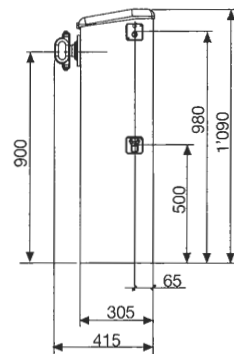
Lateral view photoelectric cell side
