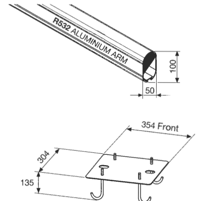
Anchor plate 354x304 with M14x200 log bolts
