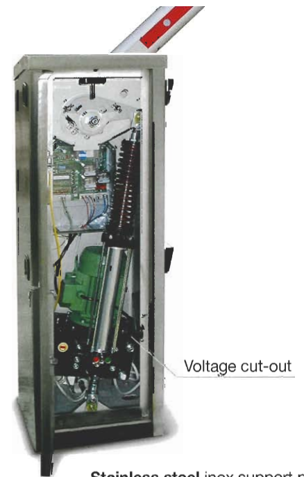
Stainless steel inox support post
